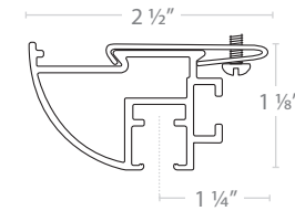
INVISIBLE CEILING CLIP
