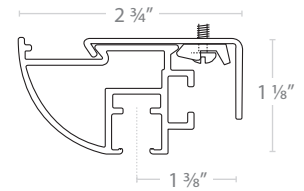
INVISIBLE SHORT PROJECTION SUPPORT
