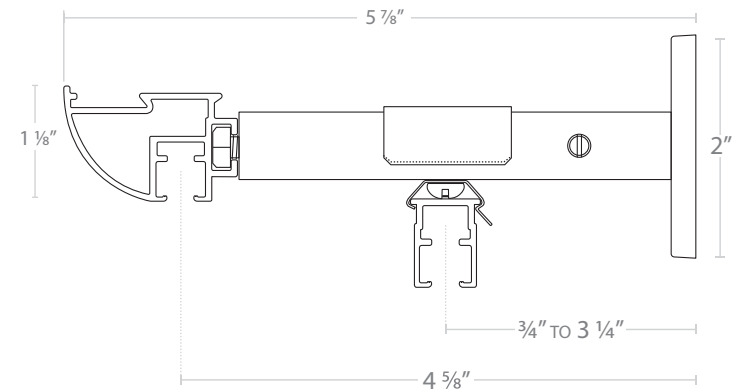
INVISIBLE TEKNO 4" PROJECTION WITH EURO SCOPE UPGRADE for Tekno 6" projection - add 2" for measurements from wall
