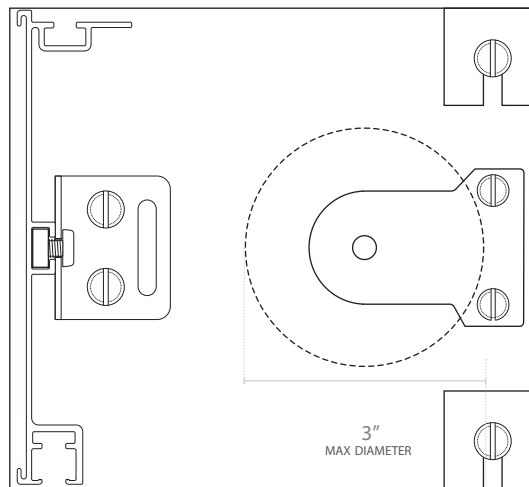
URBAN 5 - RETURN 5.5 Shade installation
