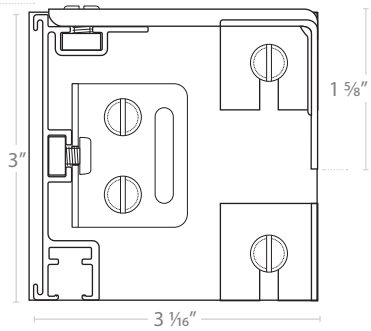
URBAN 3 RETURN 3 Showing all hardware
